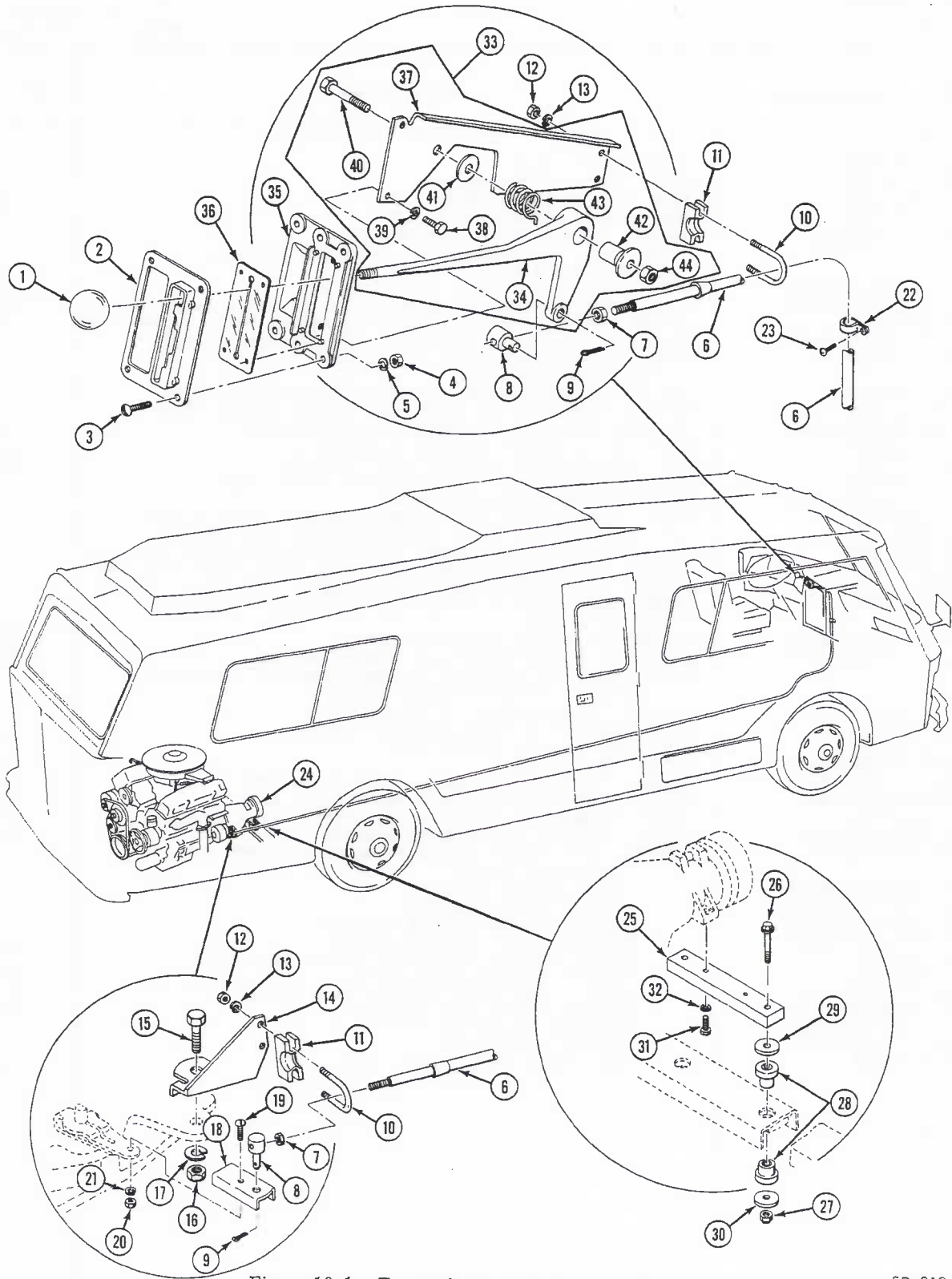
Figure 16-1. Transmission Mounting and Linkage
