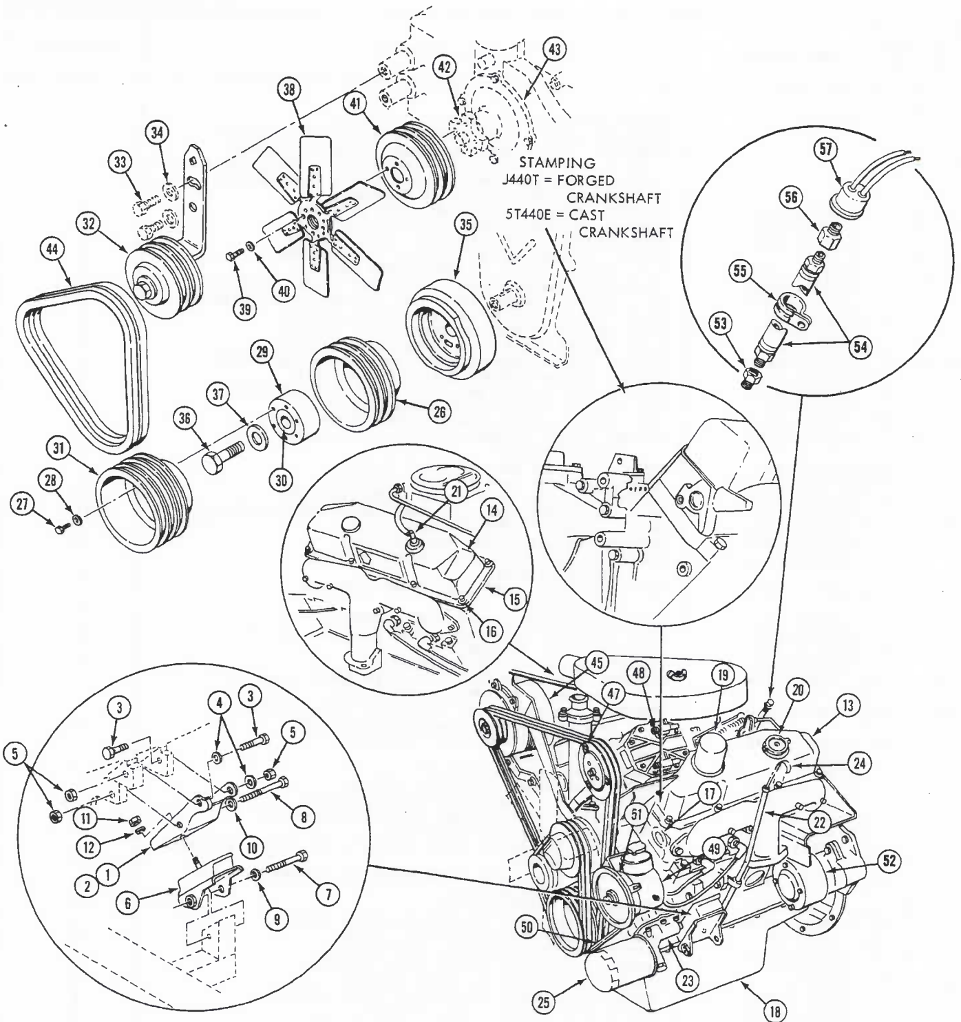
Figure 15-1. Engine Assembly
